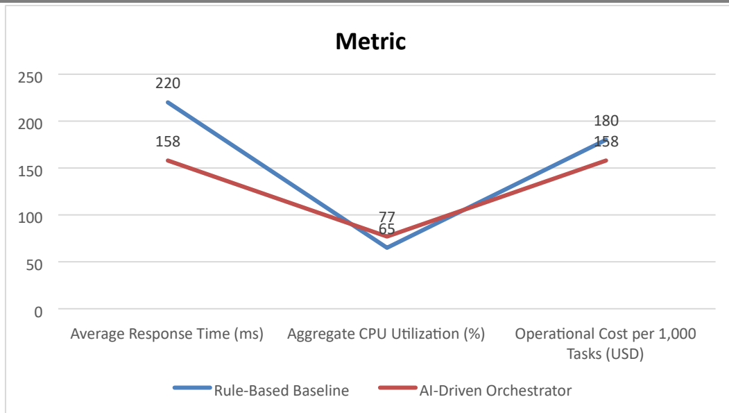
Figure-3. Comparative Metrics over 30 Runs
